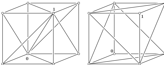
Fig. 1: Left: the Freudenthal triangulation of the 3-cube consisting of six tetrahedra sharing the edge that connects \mathbf{0} with \mathbf{1} . Right: the slice decomposition of the 3-cube consisting of two tetrahedra sandwiching an octahedron.
