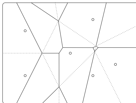
■ Figure 1 The dotted edges decompose the plane into the order-1 Voronoi domains, while the solid edges decompose it into order-2 Voronoi domains. Observe that the two tessellations share some of their vertices but not all.
