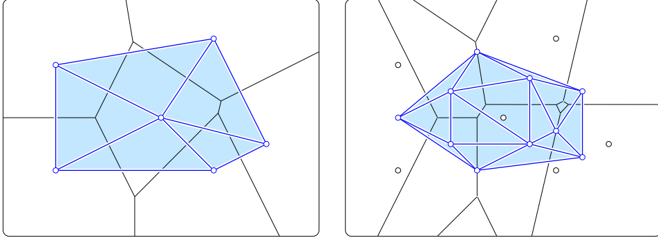
■ Figure 2 The order-1 Delaunay mosaic on the left and the order-2 Delaunay mosaic on the right , both superimposed on their corresponding Voronoi tessellations.
