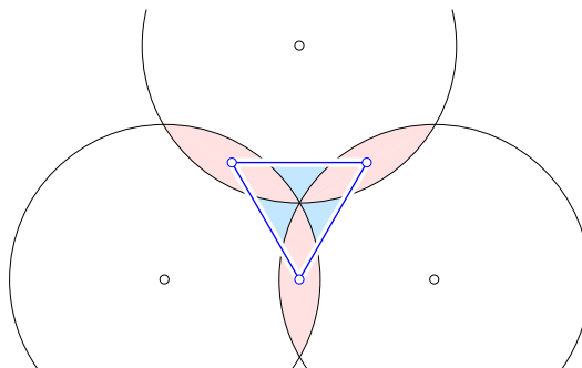
■ Figure 4 The radius function partitions the order-2 Delaunay mosaic of the three points into four relaxed intervals: three contain a vertex each, and the fourth relaxed interval contains the triangle together with its three edges.
