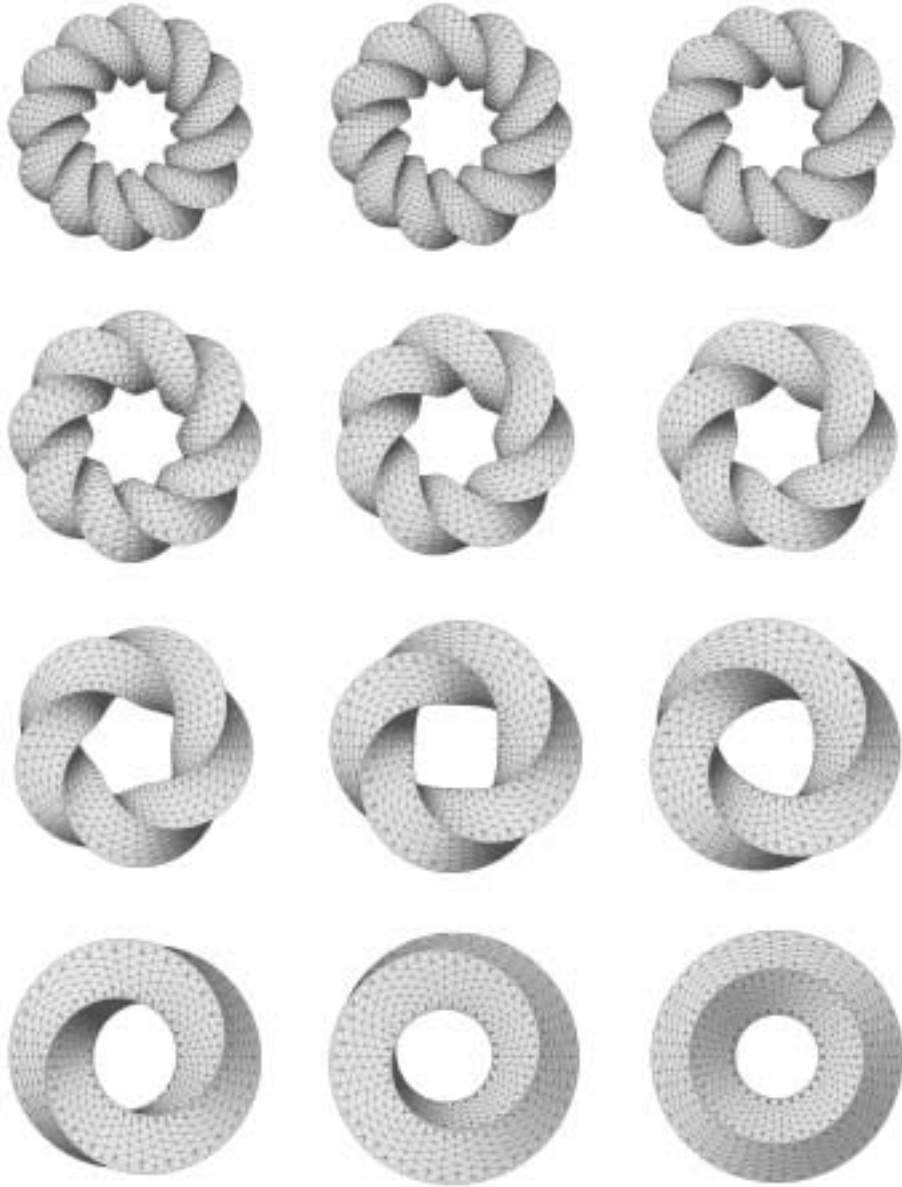
Figure 3: Square sweeping along circle in space. From left to right and top to bottom: the square rotates -\frac{12}{4} , -\frac{11}{4} , -\frac{10}{4} times, -\frac{8}{4} , -\frac{7}{4} , -\frac{6}{4} times, -\frac{5}{4} , -\frac{4}{4} , -\frac{3}{4} times, and -\frac{2}{4} , -\frac{1}{4} , 0 times.
