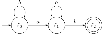
Fig. 1. A reachability game G .
