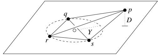
Figure 1: Y is the radius of the circle passing through q, r, s and D is the distance of p from the plane of that circle.
