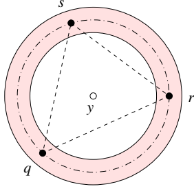
Figure 4: Every triangle qrs that forms a tetrahedron with p defines a forbidden region inside a torus of points around the circumcircle of qrs .
