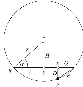
Figure 3: The circumsphere (z, Z) of pqr and the circumcircle (y, Y) of qrs projected along a direction in the plane of qrs .
