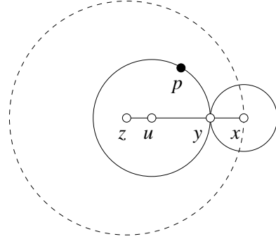
Figure 2: The solid spheres are empty of points in S and the dashed sphere is empty of points in S' .
