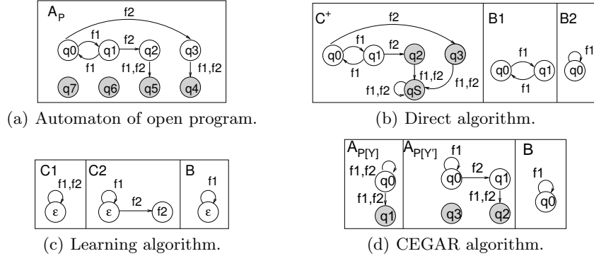
Fig. 2. Example concrete open program and the output of the three algorithms.
